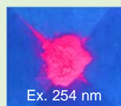
Ex. 254 nm
